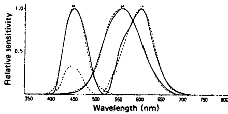
Spectral Sensitivity of Photoreceptors in Chroma Mode (Dotted line shows CIE tristimulus values.)
