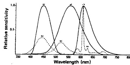
Spectral Sensitivity of Photoreceptors in Analyzer Mode (Dotted line shows spectral distribution of sample TV monitor.)
